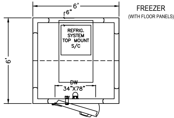
PLAN VIEW LEFT HINGE
