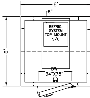
PLAN VIEW RIGHT HINGE
