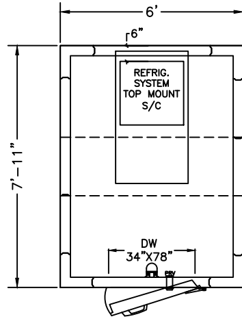
PLAN VIEW RIGHT HINGE
