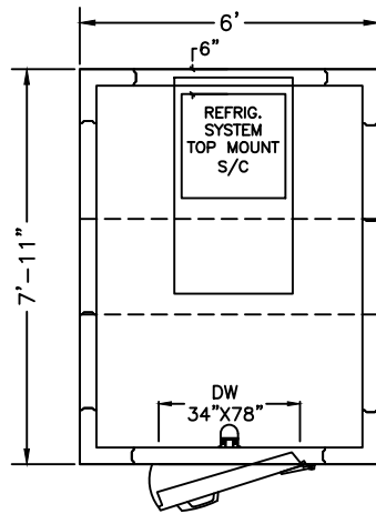
PLAN VIEW RIGHT HINGE
