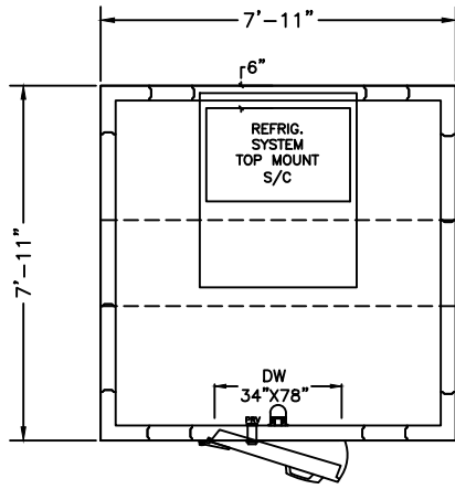
PLAN VIEW LEFT HINGE
