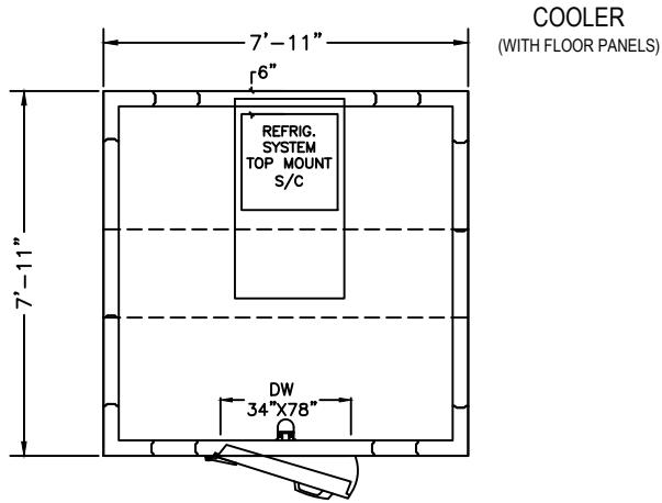
PLAN VIEW LEFT HINGE
