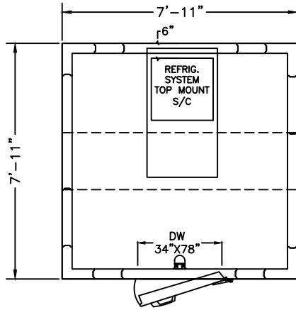
PLAN VIEW RIGHT HINGE
