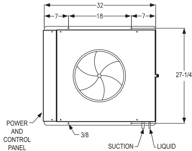
Figure 1 - Single Fan
