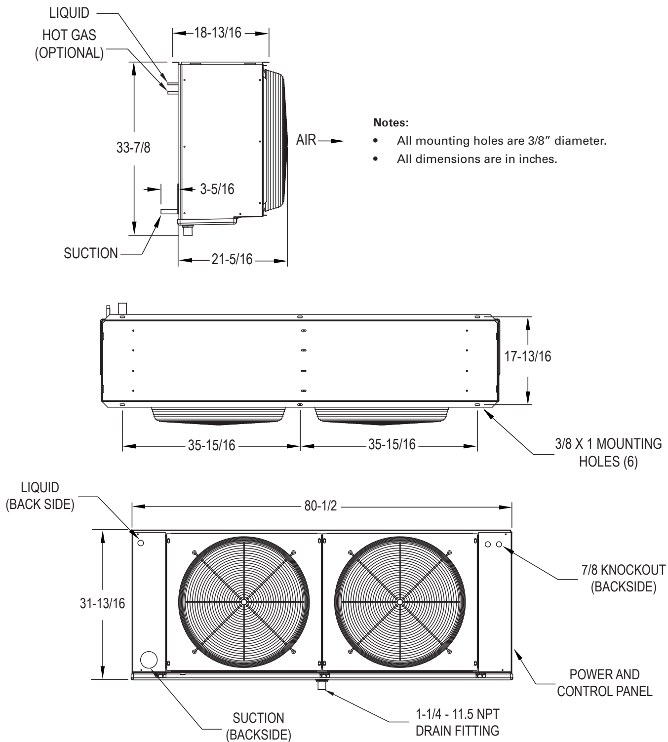
Figure 2- Two Fan
