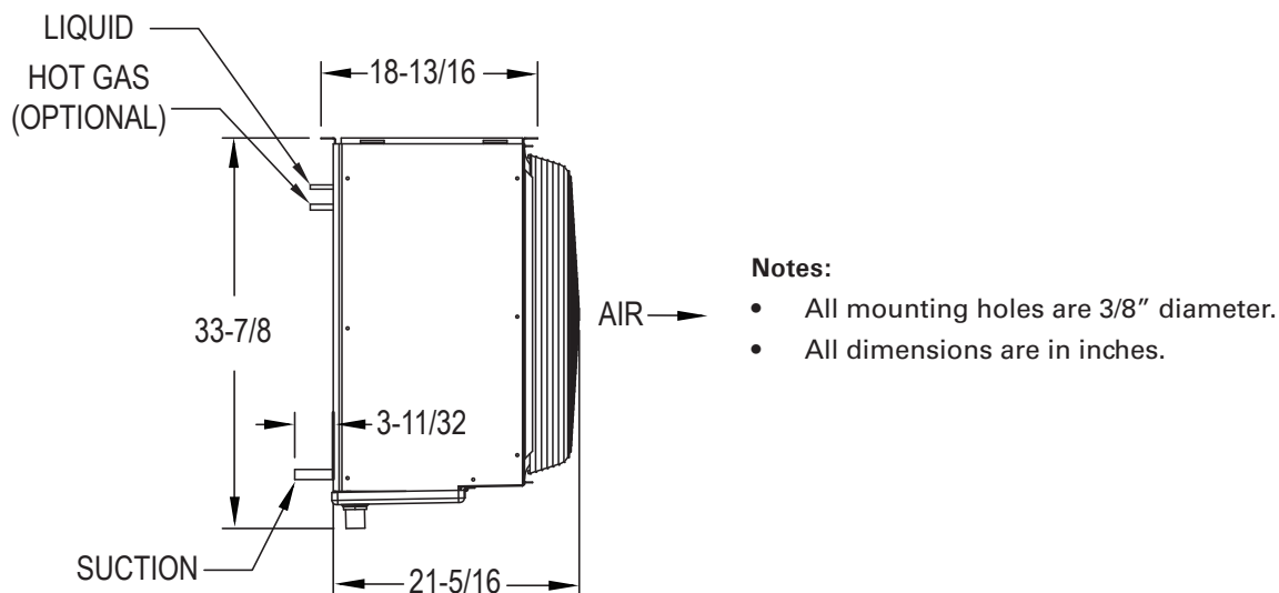
Figure 1 - Single Fan
